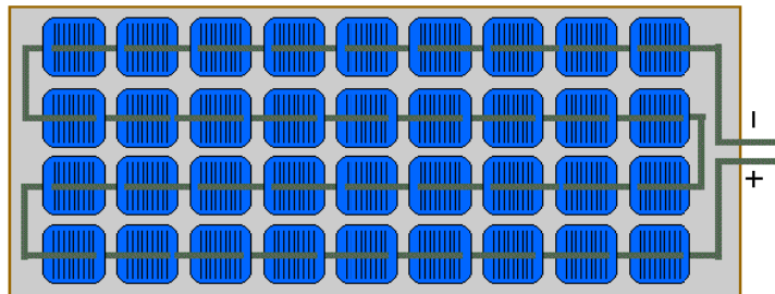
A typical module has 36 cells in series
